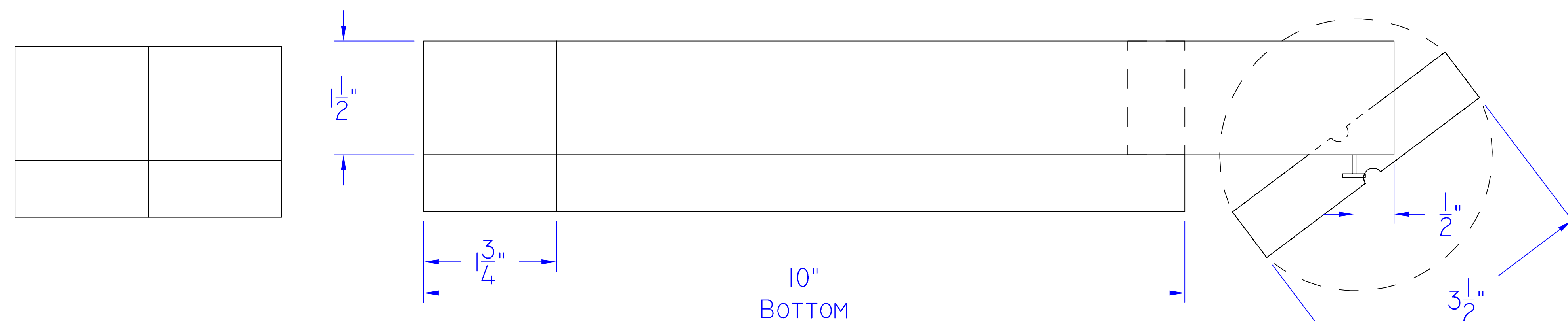
Front View
