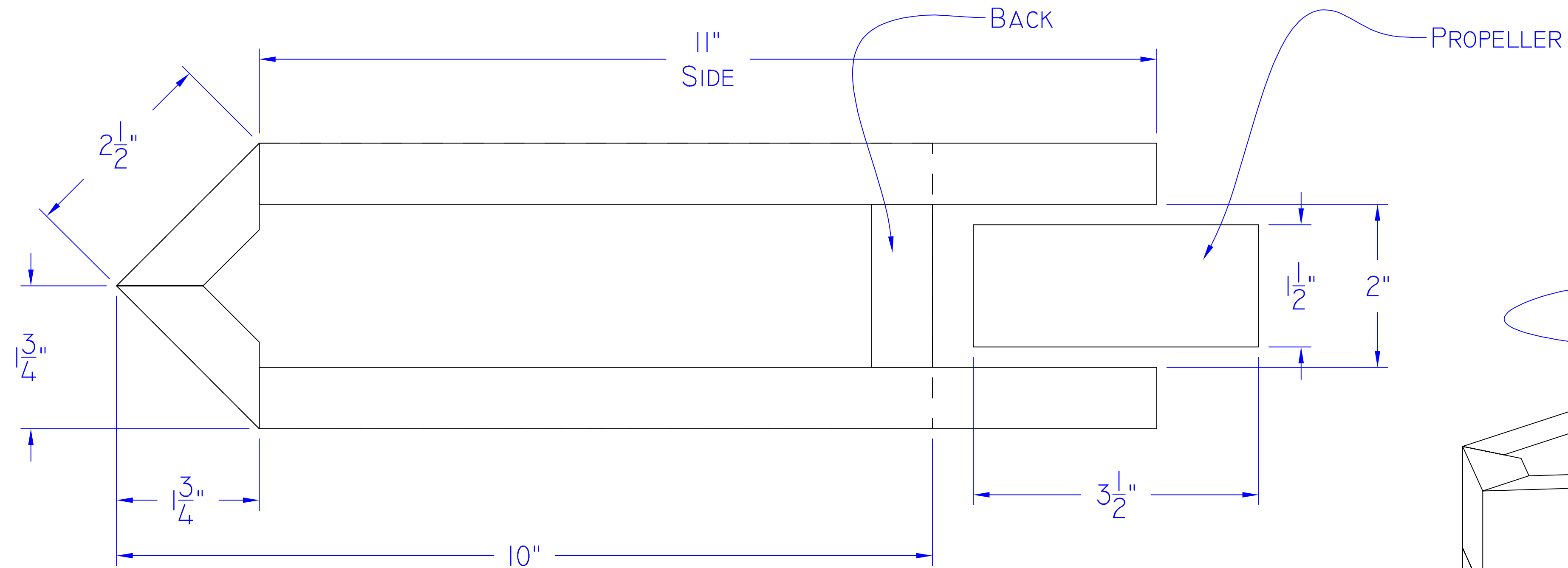
Top View
